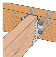
Hanger connection
